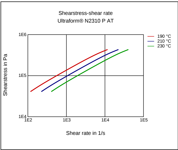
Shearstress-shear rate
