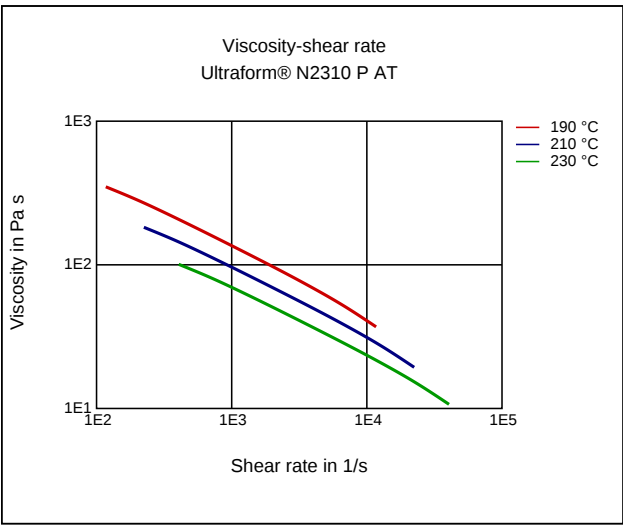
Viscosity-shear rate
